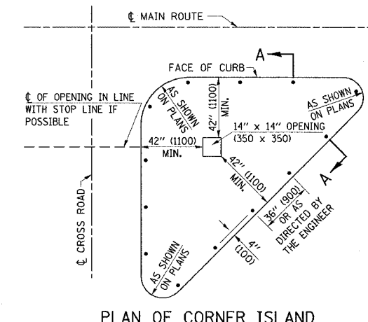
PLAN OF CORNER ISLAND
