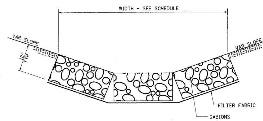
DETAIL OF GABIONS
