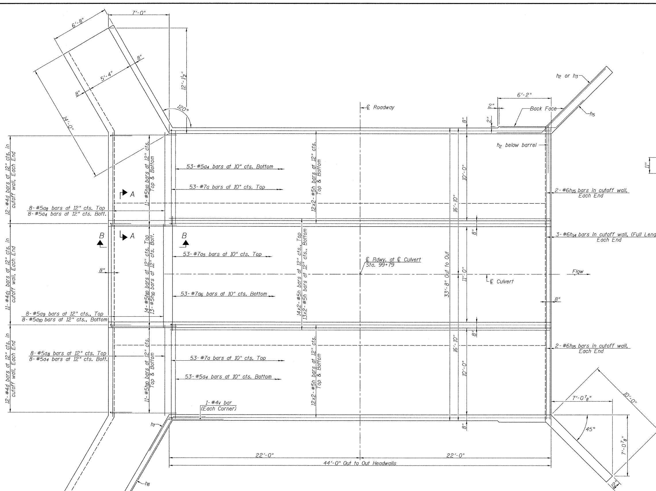
PLAN (Bottom Slab)
