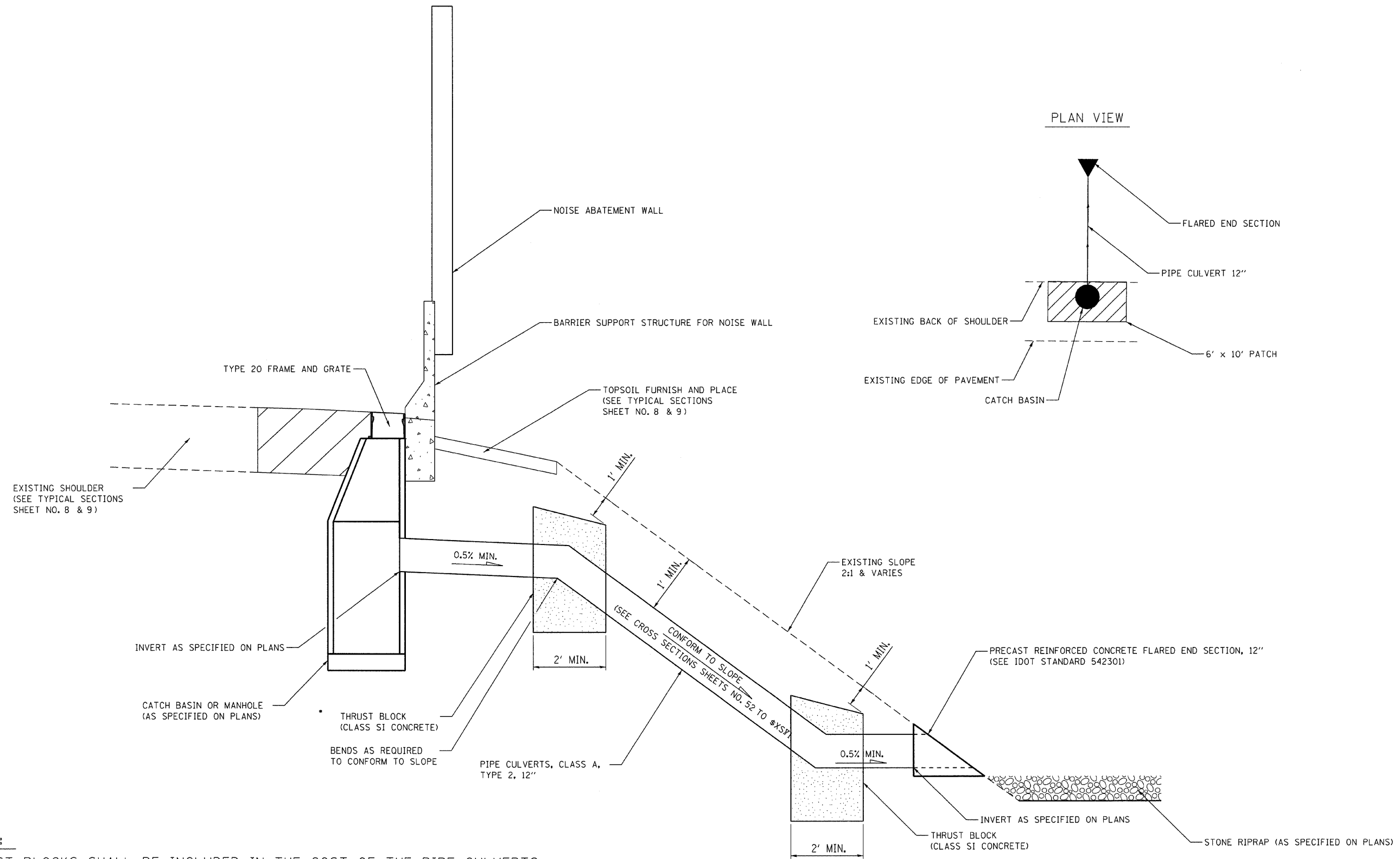
DRAINAGE DETAIL
