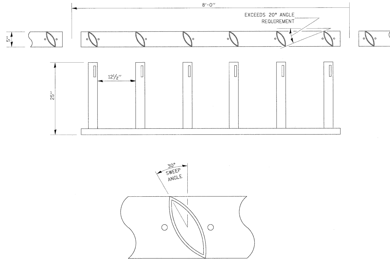
DETAIL DRAWING
