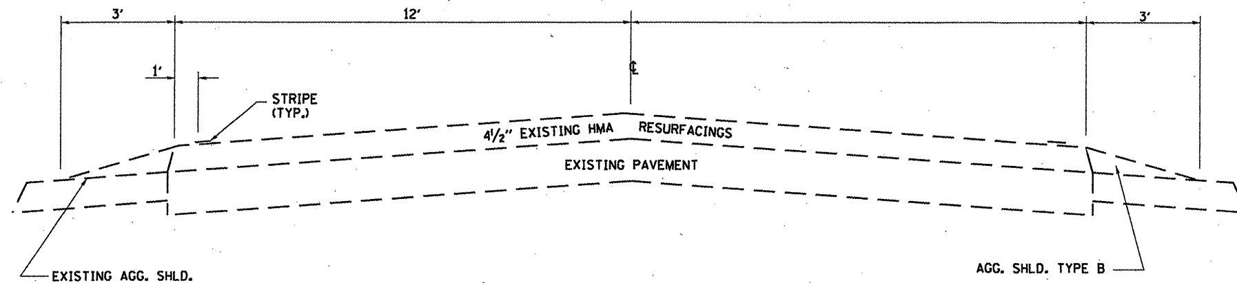
TYPICAL SECTION
