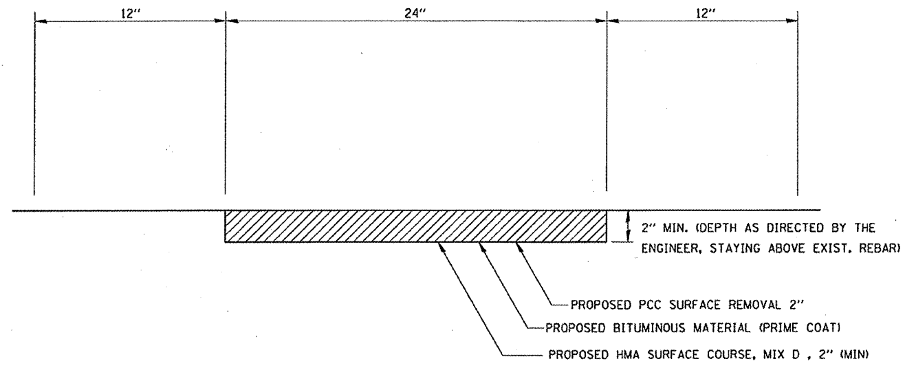
(TYPICAL) PROPOSED LONGITUDINAL JOINT REPAIR DETAIL
