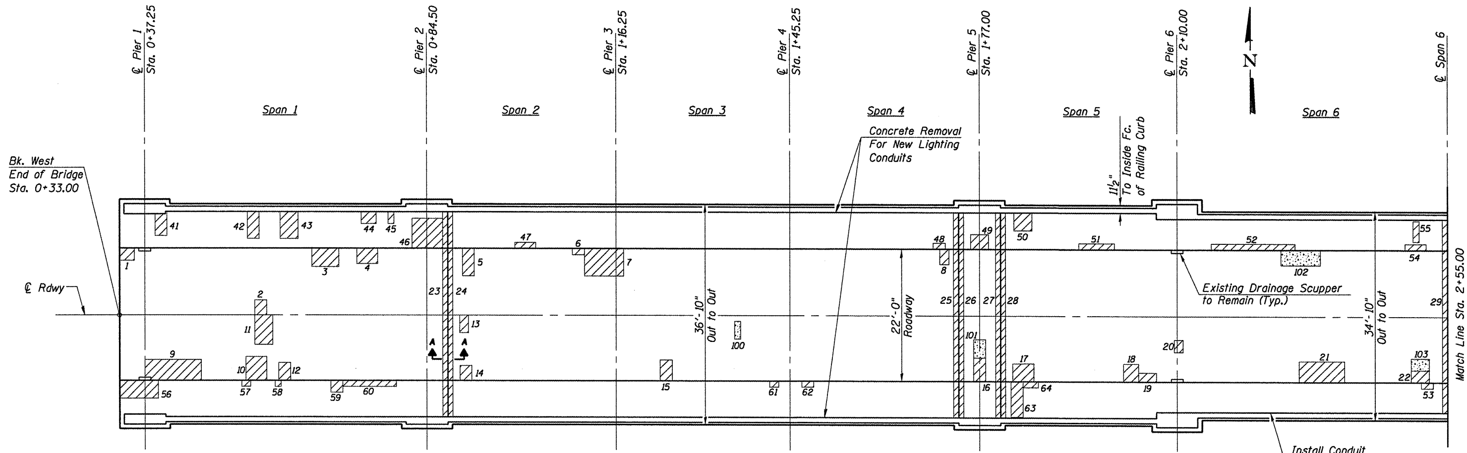
DECK REPAIR PLAN (Spans 1 thru 6)
