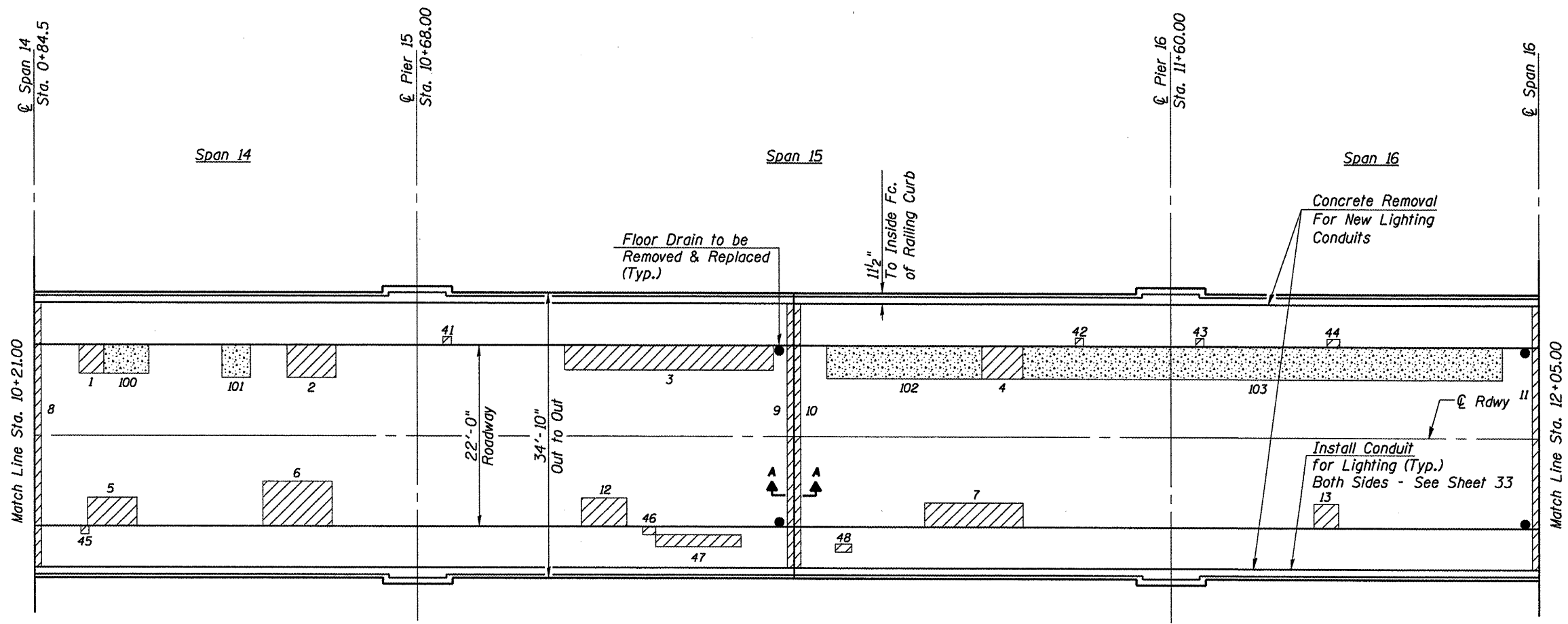
DECK REPAIR PLAN (Spans 14 thru 16)
