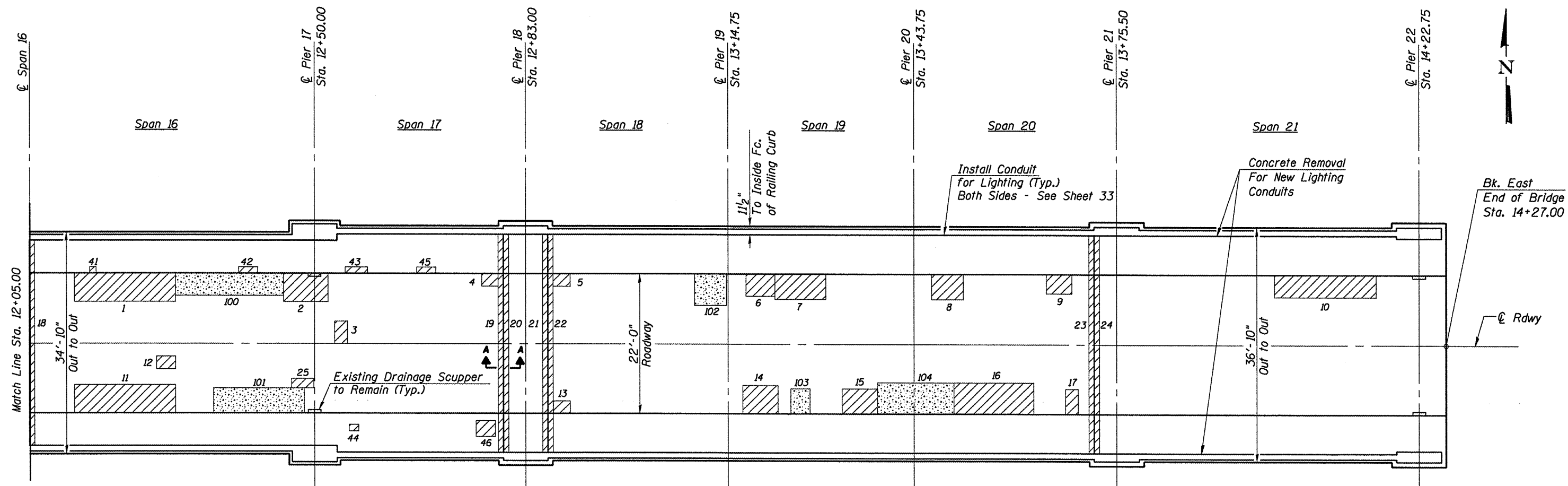
DECK REPAIR PLAN (Spans 16 thru 21)
