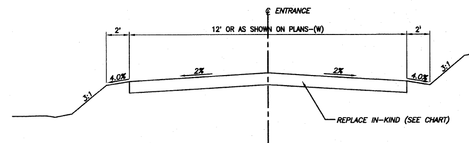
SECTION "D-D"
