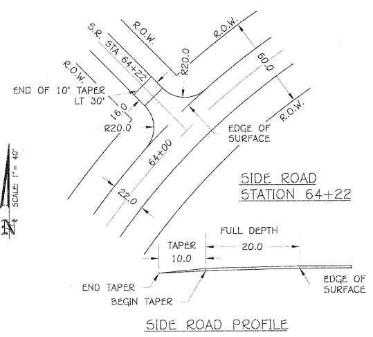
HOT-MIX ASPHALT SURFACE COURSE, MIX "C", N50 = 14.00 TON (INCLUDED)
