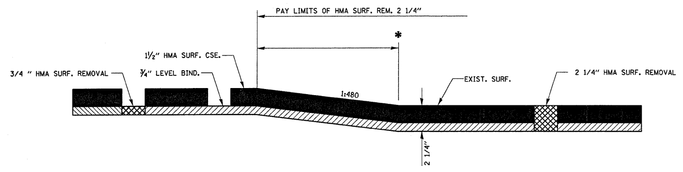
TRANSITION FROM HMA SURF. REM. 3/4" TO HMA SURF. REM. 2 1/4"
