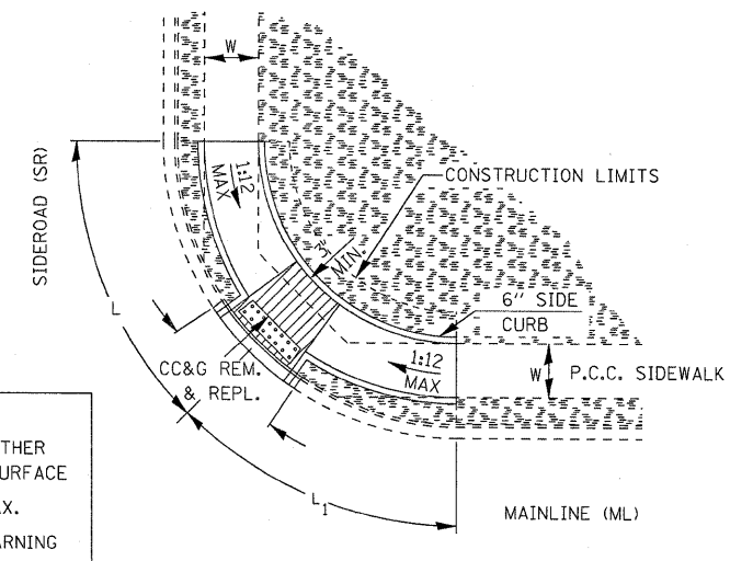
ADA SIDEWALK ACCESSIBILITY RAMPS METHOD 6
