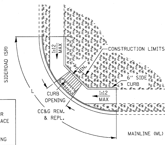
ADA SIDEWALK ACCESSIBILITY RAMPS METHOD 6
