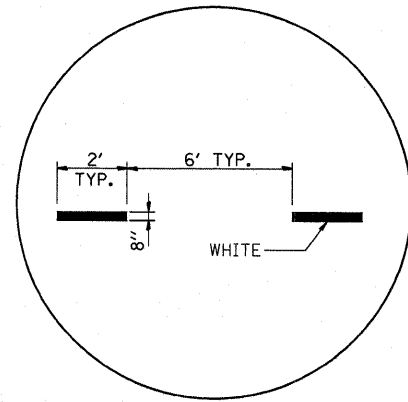
DETAIL FOR TURN LANE DASHED
