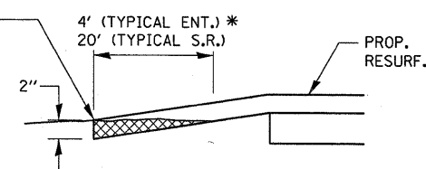
DETAIL A
