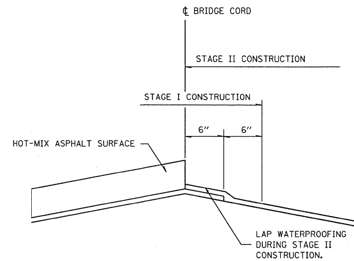
WATERPROOFING DETAIL
