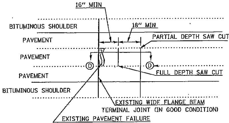
PAVEMENT SAWING DETAIL
