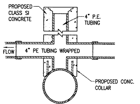
TYPE C INSPECTION HOLE DETAIL "NOT TO SCALE"
