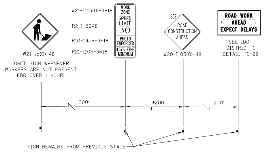
ADVANCE SIGNING FOR BROOKDALE ROAD (SPACING MAY VARY DUE TO FIELD CONDITIONS)
