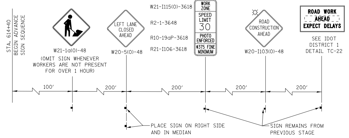
ADVANCE SIGNING FOR WESTBOUND DIEHL ROAD (SPACING MAY VARY DUE TO FIELD CONDITIONS)
