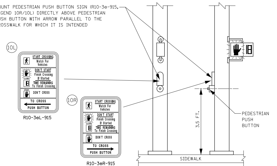
PEDESTRIAN PUSH BUTTON SIGN MOUNT DETAIL
