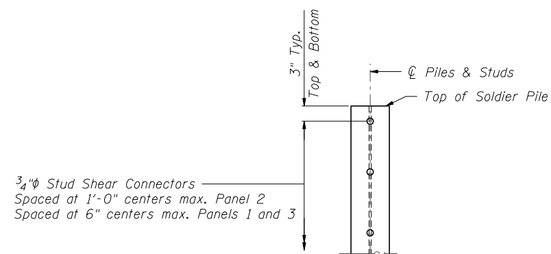
DETAIL OF SHEAR STUD PLACEMENT
