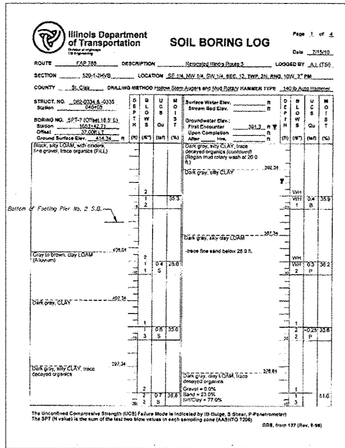
BORING SPT-7 (1 of 4)
