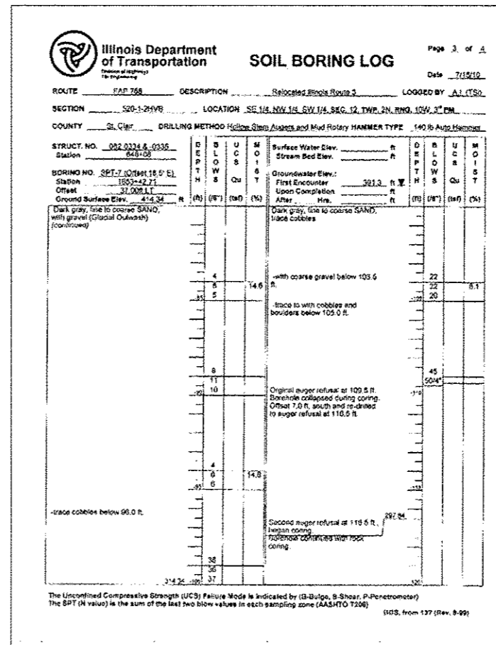
BORING SPT-7 (3 of 4)
