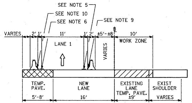
PP-PP STAGE 3: WB CONNECTOR; STA. 337+38 TO STA. 340+29
