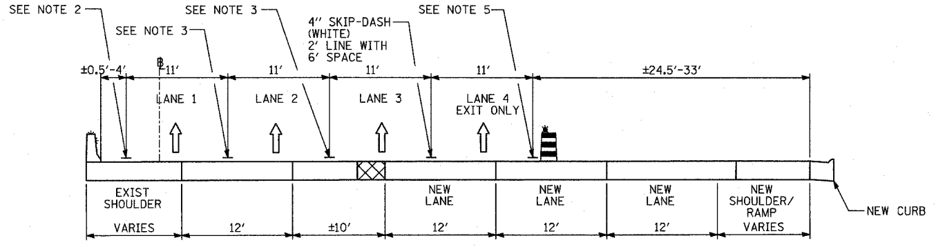
LL-LL STAGE 2: NB I-94 (DAN RYAN); STA. 2229+78 TO STA. 2236+13
