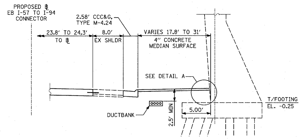
SHOULDER DETAIL AT STATE STREET
