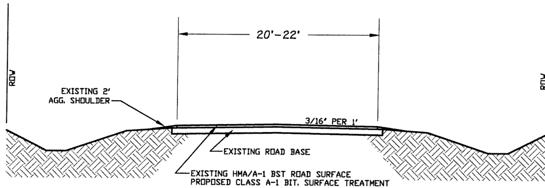
TYPICAL CROSS SECTION OF EXISTING/PROPOSED ROAD
