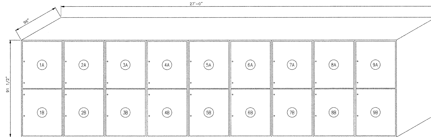
5KV SWGR ELEVATION CONTROL ROOM
