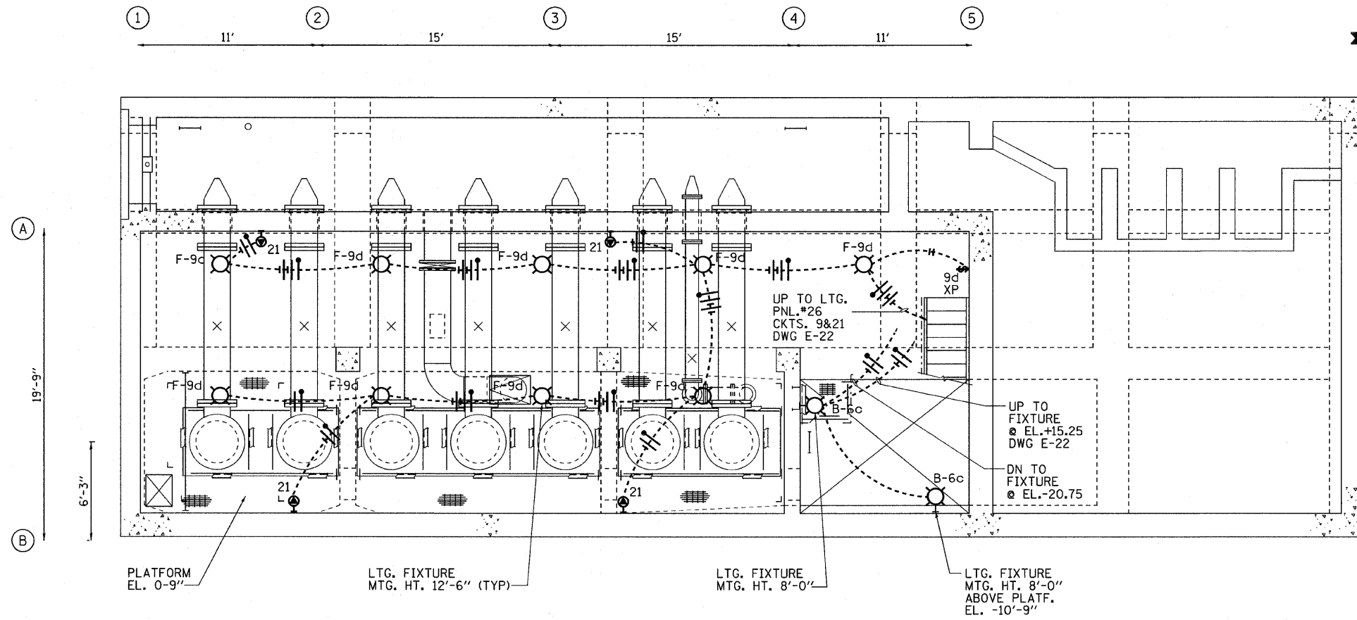
PLAN B-B AT EL.-2.75'
