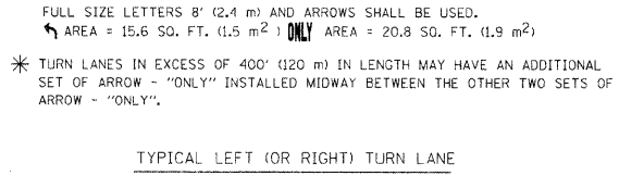
TYPICAL TURN LANE MARKING
