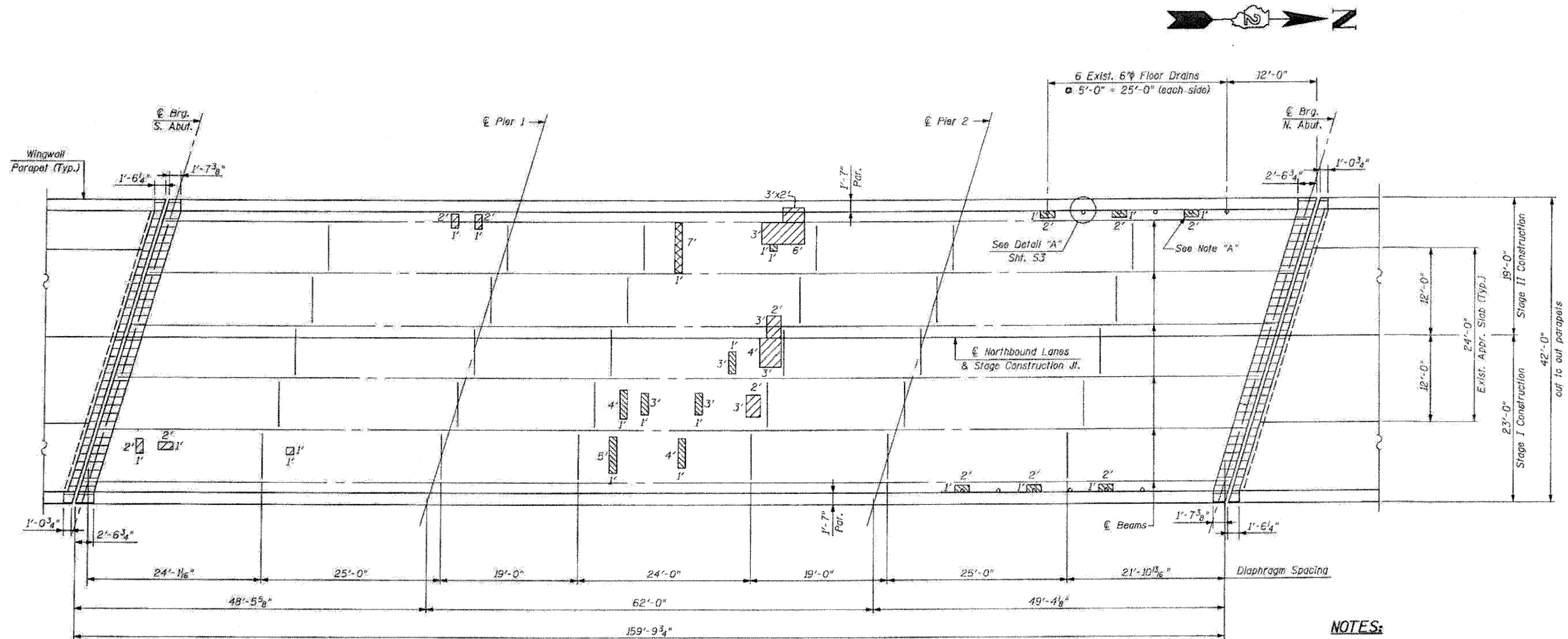
DECK PLAN
