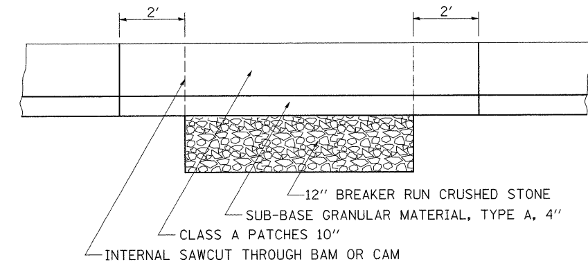
CLASS A PATCHES WITH DRAINS FOR AGG BASE COURSE
