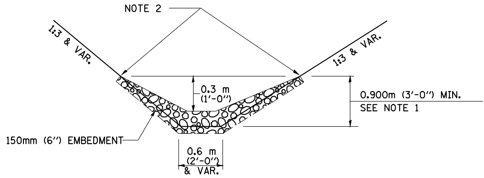
ELEVATION OPTION 1
