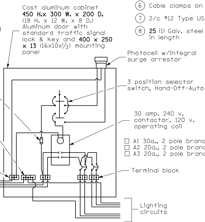
WIRING DIAGRAM
