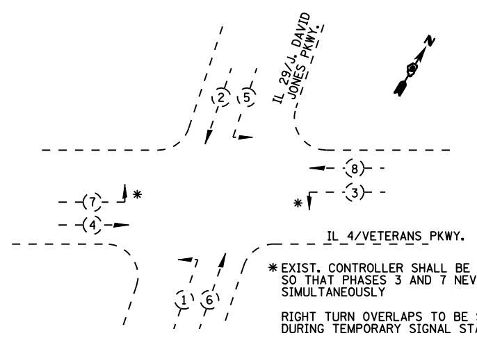
TEMPORARY SIGNAL PHASE DESIGNATION DIAGRAM
