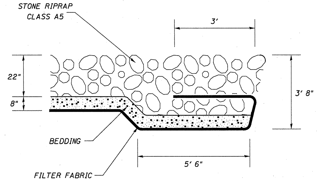
RIPRAP TOE DETAIL
