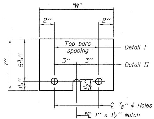
STEEL RETAINER PL 1" x 7" x 10"
