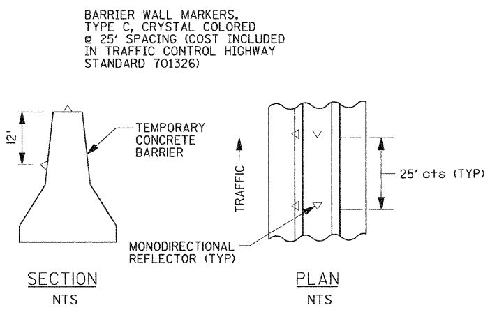
BARRIER WALL REFLECTORS DETAIL FOR TEMPORARY CONCRETE BARRIER
