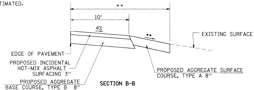
ENTRANCE DETAILS
