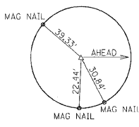
POT STA 106+52.89 (P.K. NAIL)
