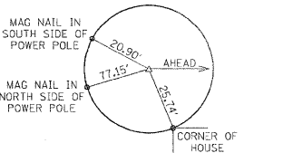
POT STA 3+00.00 (ALLEY @ STA 149+27.00) = (MAG NAIL)
