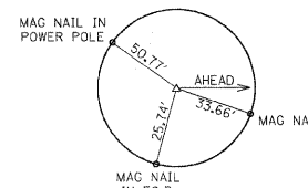
POT STA 15+43.67 (S LOOP ST) (P.K. NAIL)
