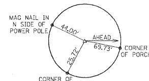
PT STA 156+97.64 (P.K. NAIL)
