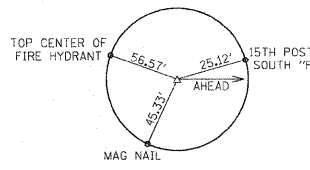
PT STA 19+59.24 (S LOOP ST) (IRON PIN W/CAP)
