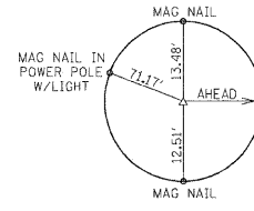
PC STA 143+28.62 (P.K. NAIL)
