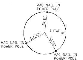
PCC STA 17+98.78 (S LOOP ST) (MAG NAIL)
