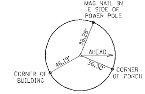
PC STA 157+33.68 (P.K. NAIL)
