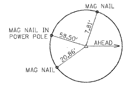
PT STA 2+68.26 (MCKINLEY AVE) (P.K. NAIL)
