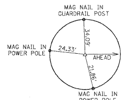
POT STA 0+00.00 (N LOOP ST) = ML STA 144+68.00 (P.K. NAIL)
