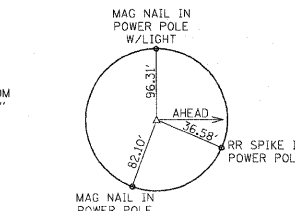
POT STA 20+00.00 (S CHESTNUT ST) = ML STA 134+35.00 (P.K. NAIL)
