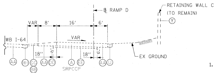
EXISTING RAMP "D" TO BE REMOVED (SHOWN FOR INFORMATION ONLY)
