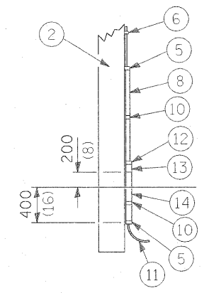
POLE, WOOD
