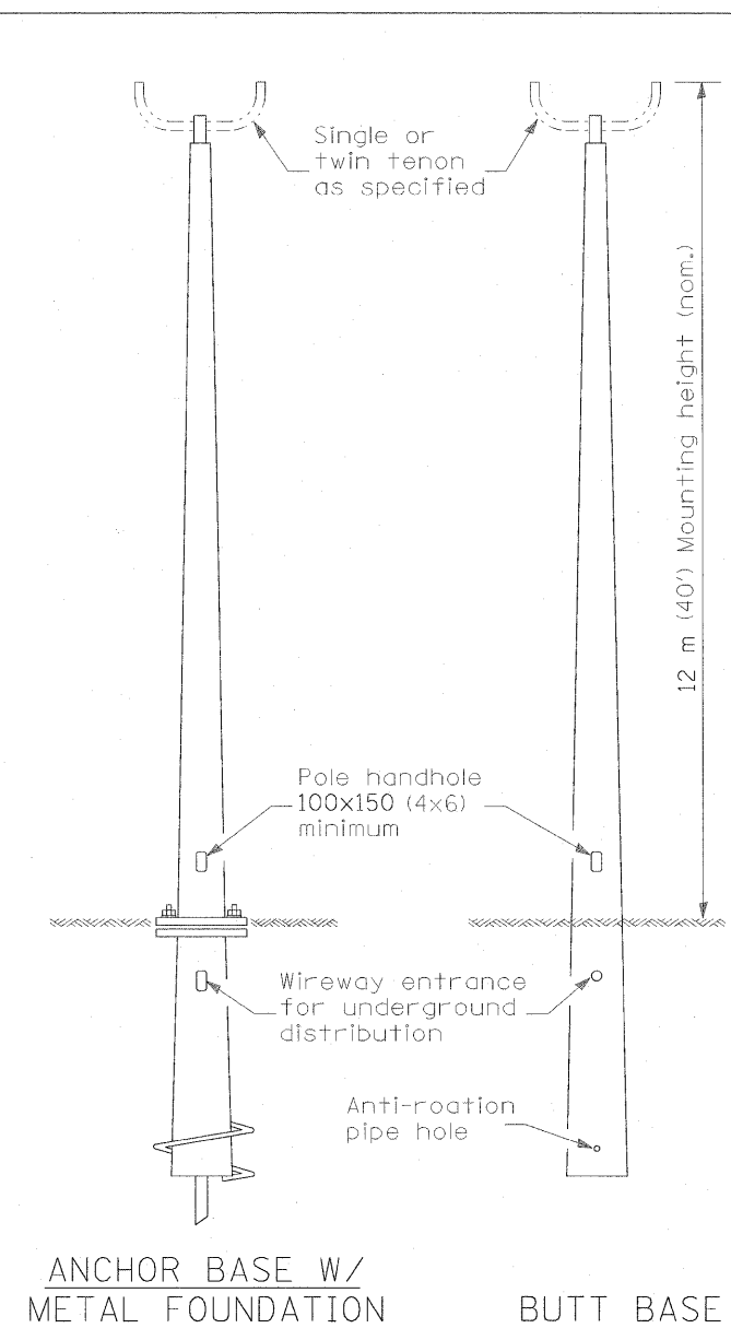
POLE, FIBERGLASS BREAKAWAY TYPE
