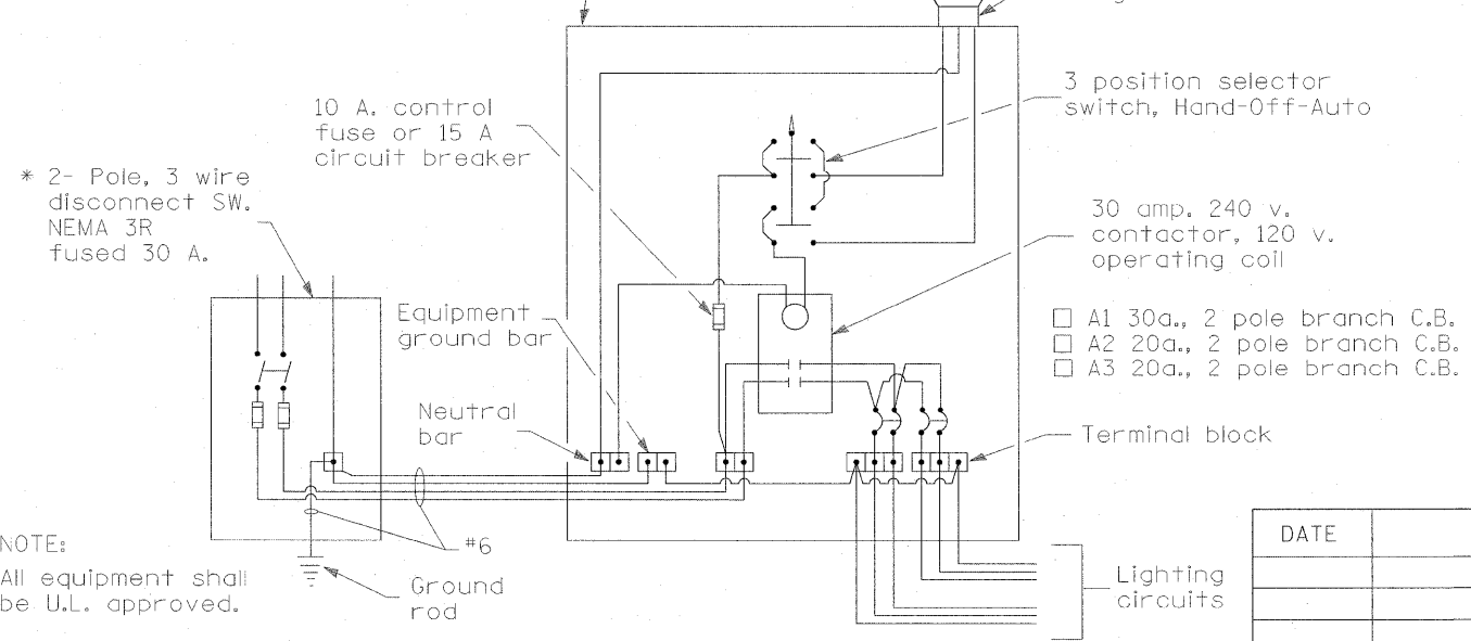
WIRING DIAGRAM
