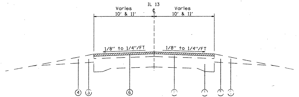
EXISTING TYPICAL SECTION FAU 9251 (IL 13) STA. 109+11 to STA. 109+61
