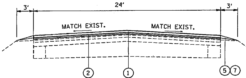
FRONTAGE ROAD 0.04 - 0.605
