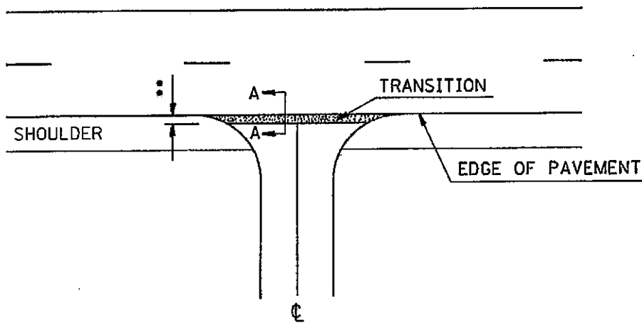
SIDEROAD DETAIL
