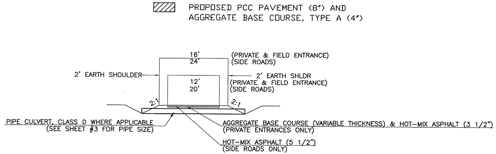
TYPICAL ENTRANCE & SIDE ROAD DETAILS
