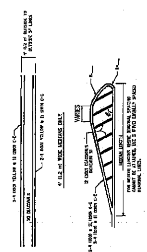
TYPICAL TURN LANE MARKING
