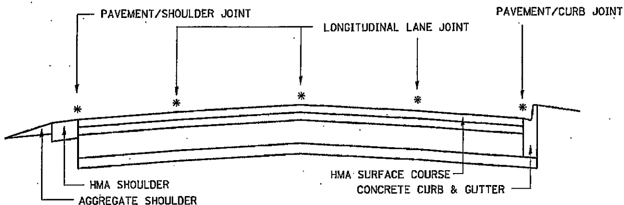
MULTI-LANE DIVIDED PAVEMENT
