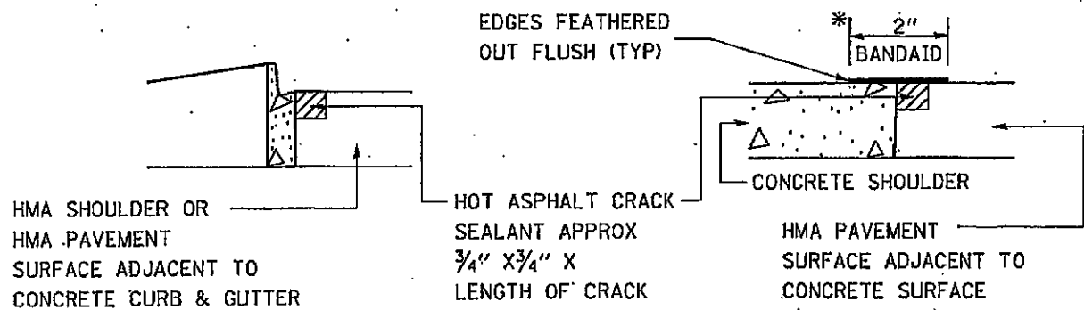
CRACK & JOINT SEALING DETAIL
