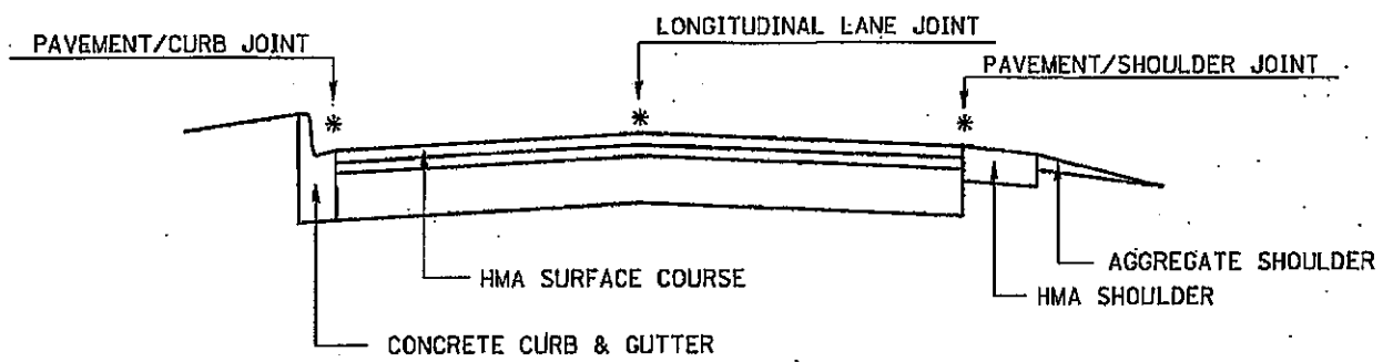
TWO-LANE PAVEMENT
