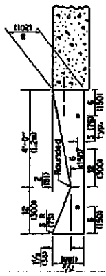
SECTION C-C
