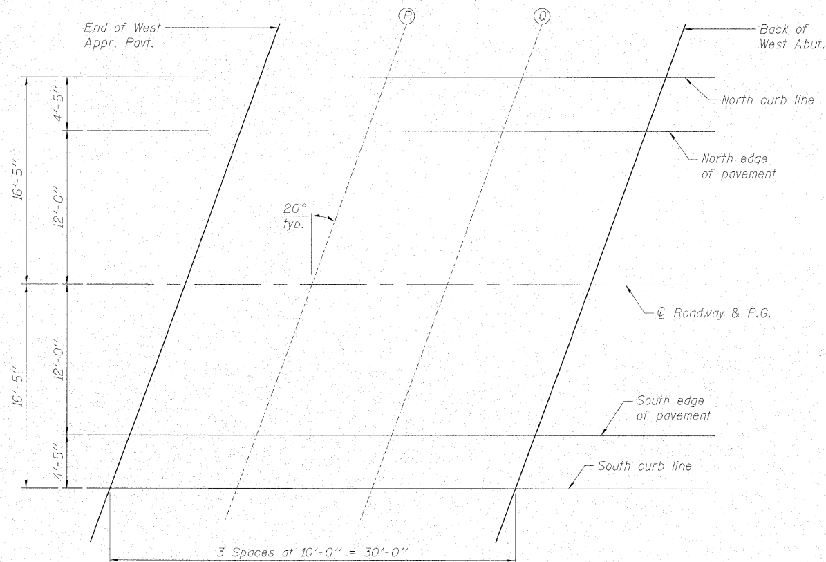
PLAN
