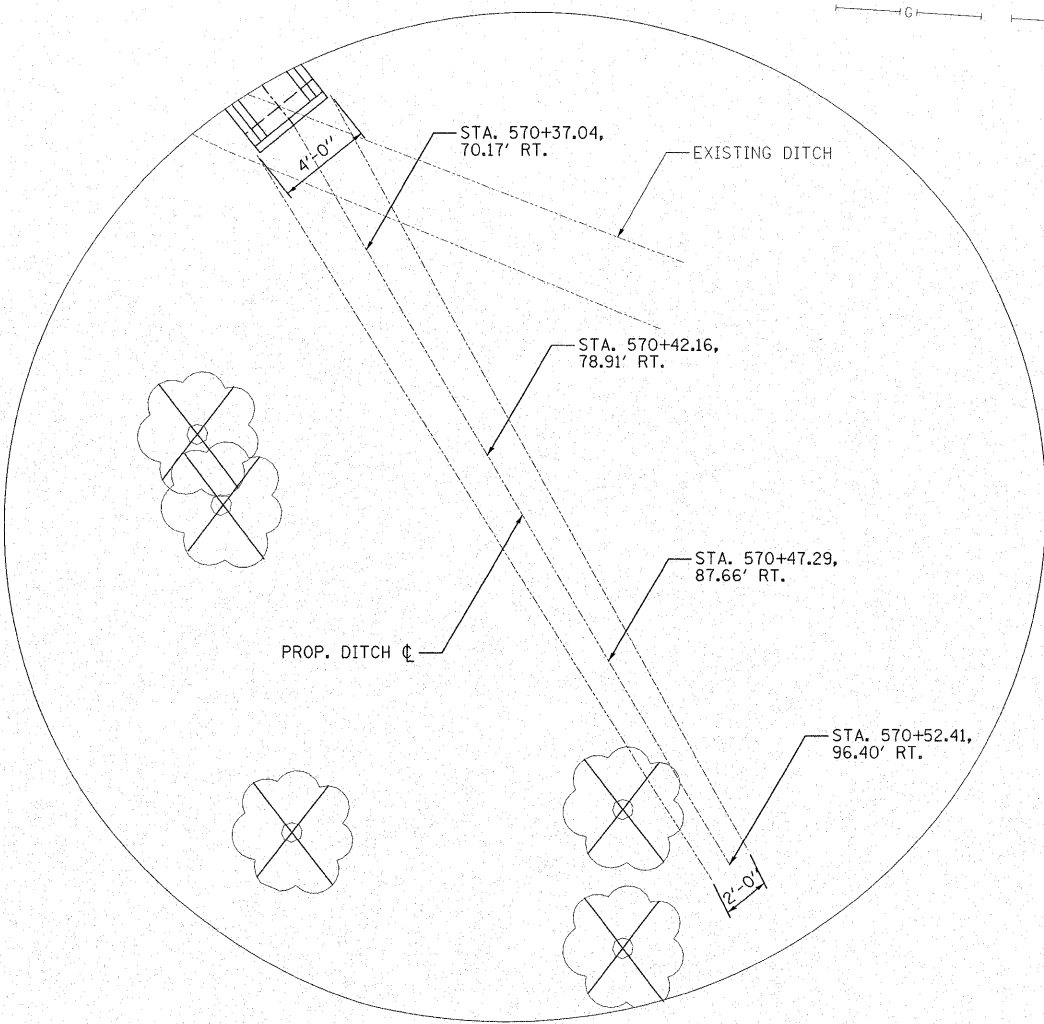
DITCH DETAIL
