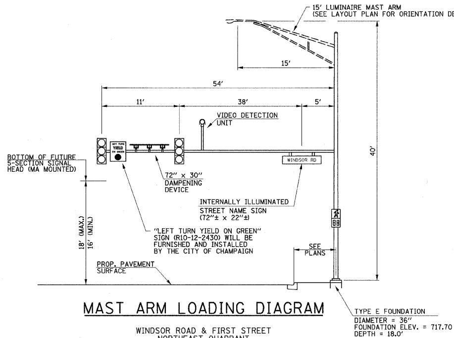
MAST ARM LOADING DIAGRAM
