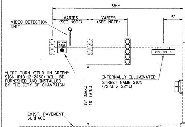
MAST ARM LOADING DIAGRAM
