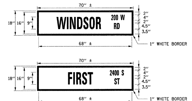
INTERNALLY ILLUMINATED STREET NAME SIGN FACE DETAILS
